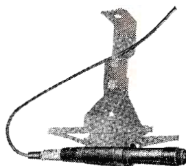
ALTEC 688A OMNIDIRECTIONAL DYNAMIC MICROPHONE —$90 net. Extremely uniform response from below 35 to over 20,000 cycles. Highly efficient. Low hum pickup. Shown in an Altec 181A Boom Mount. Output Impedance: 30/50, 150/250 and 20,000 ohms (selection by connections in microphone cable plug). Output Level: -55 dbm/10 dynes/cm 2 . Hum: -120 db (Ref.: 10 -3 Gauss). Dimensions: 1 1/8" diameter at top (1 1/2" largest diameter), 7 1/2" long not including plug. Weight: 8 ozs. (not including cable and plug).
