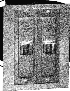
FAIRCHILD EQUALIZED NAB PLAYBACK PRE-AMP, Model 676A — a low noise silicon transistor preamp for proper NAB playback of records. Minimum controls assure consistency of station quality. Available mono — 676A; stereo — 676A-2 (pictured).
