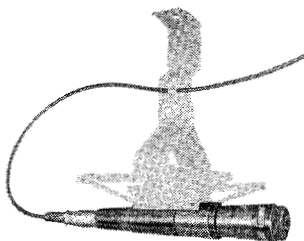
ALTEC 689A CARDIOID DYNAMIC MICROPHONE —$108 net. High front-to-back discrimination for an average of over 20 db from 40 to over 16,000 cycles. Virtually flat response throughout this frequency range. Output Impedance: 30/50, 150/250 and 20,000 ohms (selection by connections in microphone cable plug). Output Level: -54 dbm/10 dynes/cm 2 . Hum: -120 db (Ref.: 10 -3 Gauss). Dimensions: 1 1/8" diameter at top, 7 1/2" long not including plug. Weight: 11 ozs. (not including cable and plug).
